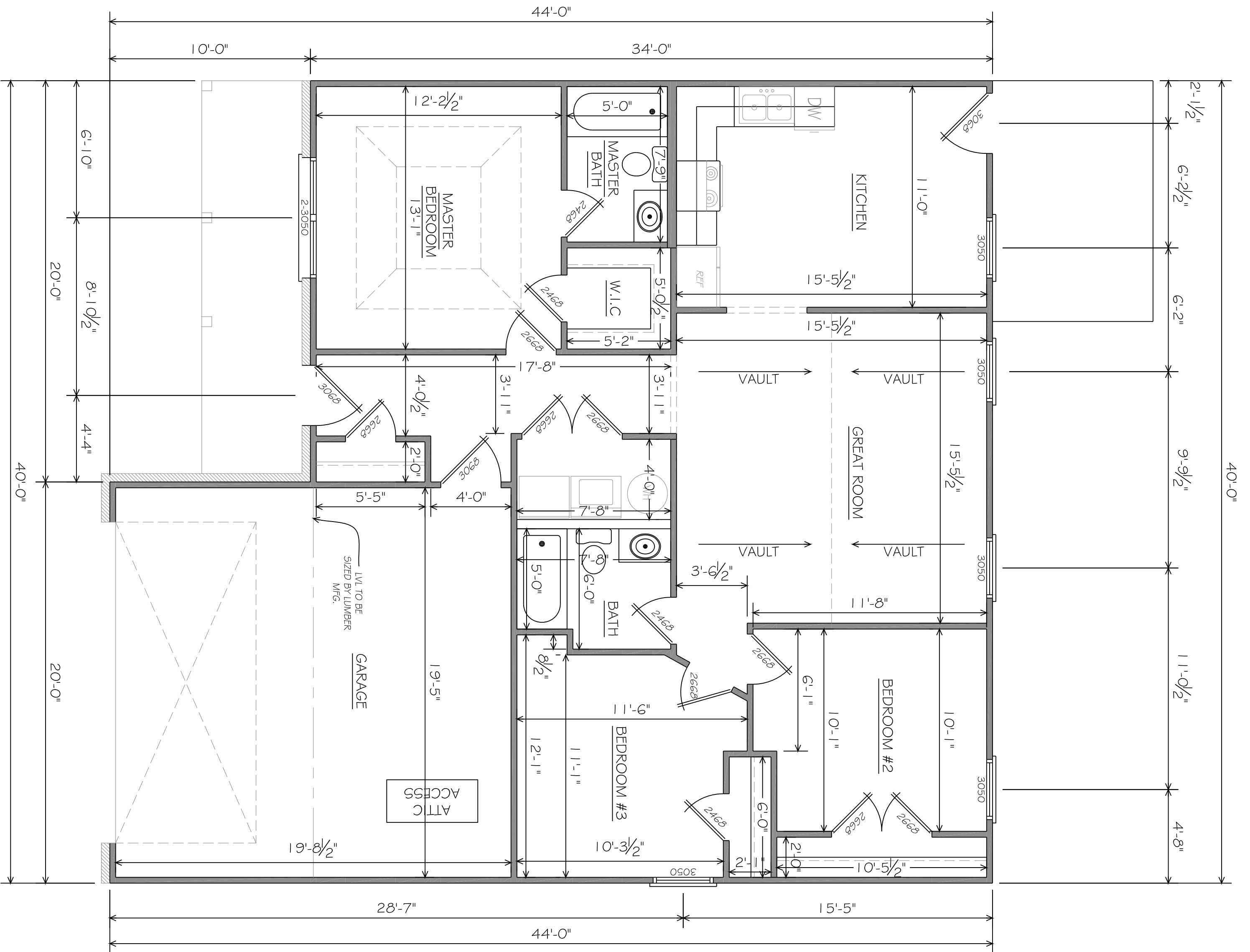
1 FLOOR PLAN SCALE: 1/4" = 1'-0" 1171 sq.ft.
