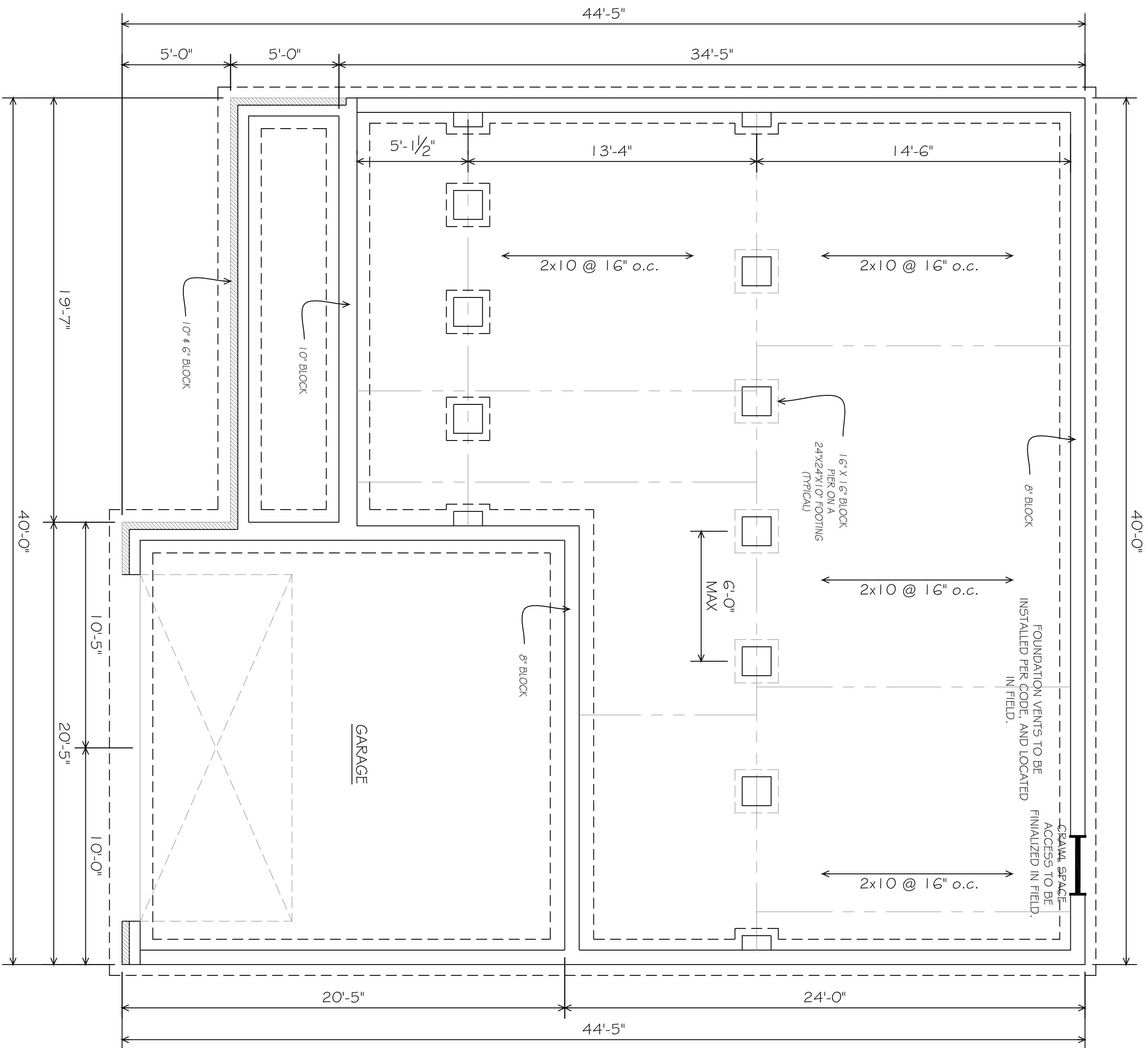
1 FOUNDATION PLAN A-1 SCALE: 1/4" = 1'-0"
